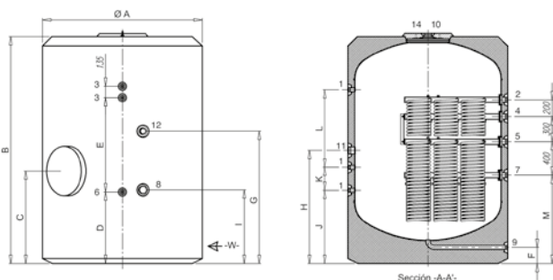
AS 2000-2E, AS 3500-2E e AS 5000-2E (2 serpentinas)
