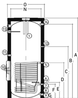
AS 750-1E e AS 1000-1E (1 serpentina)
