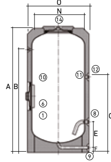
AS 1500-IN (sem serpentina)
