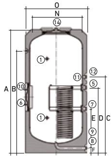
AS 1500-1E (1 serpentina)
